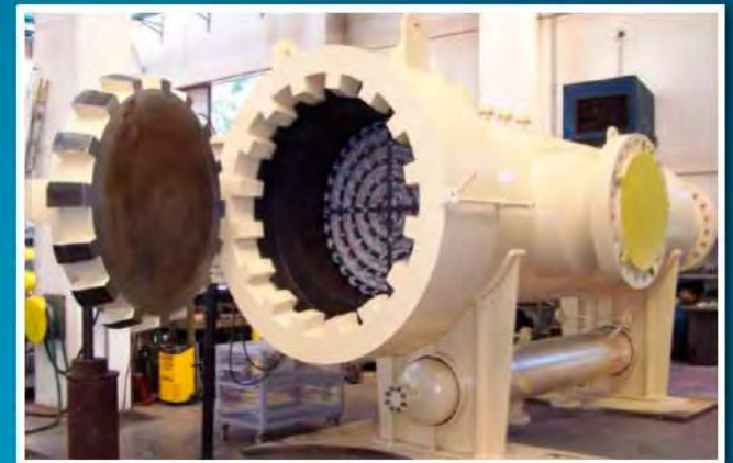
FILTER SEPARATOR FSO TYPE - 60" # 900, THK 82 mm
