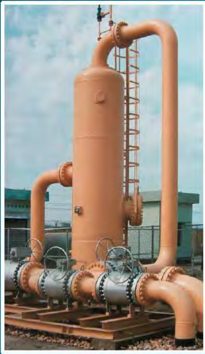
SLUG CATCHER SLV TYPE - 42" # 300
