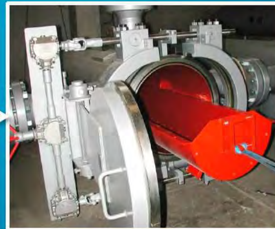
BIDIRECTIONAL TRAP 22" x 16" # 600
